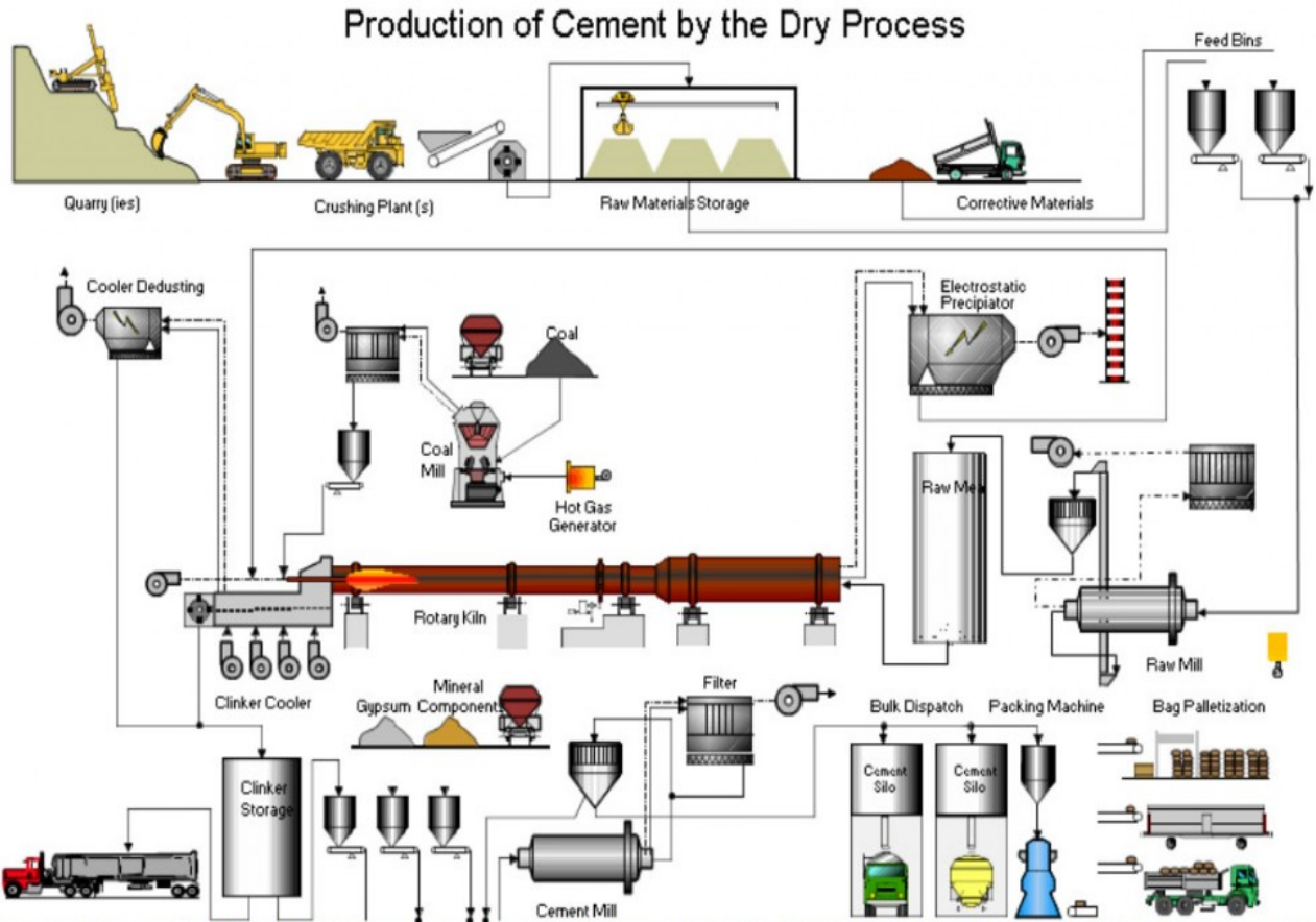
Figure 2-1: Process Flow diagram of the cement manufacturing process at Port Elizabeth. Please note that PE has long dry kiln with no preheater stage.
